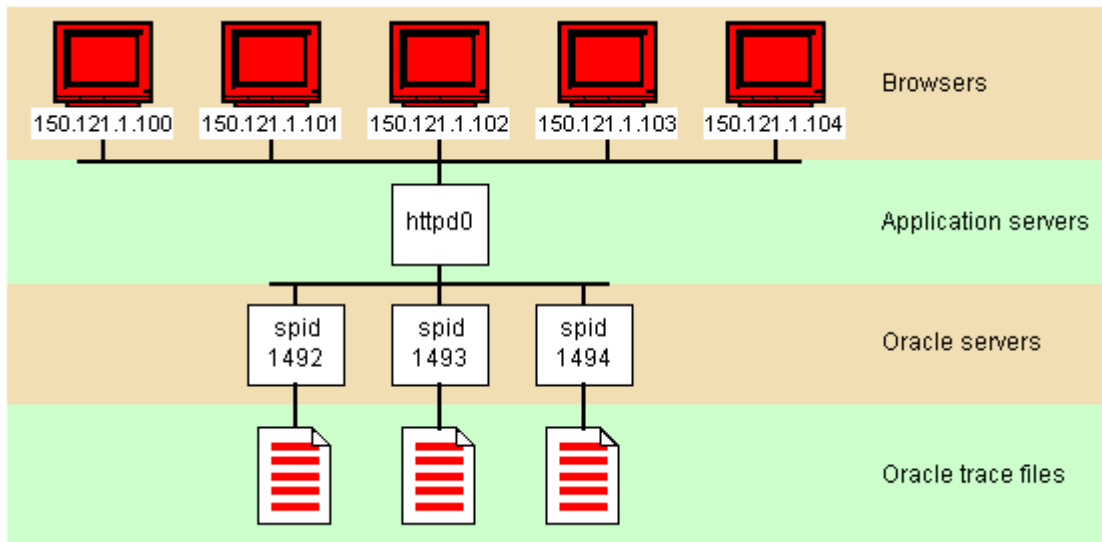
Figure 2. Aggregating across similar transactions in a connection pooling environment
